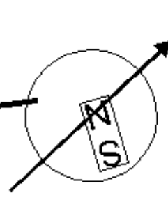
Neptune
