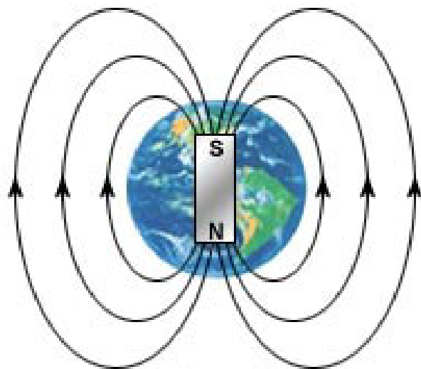
Earth's Magnetic Field
