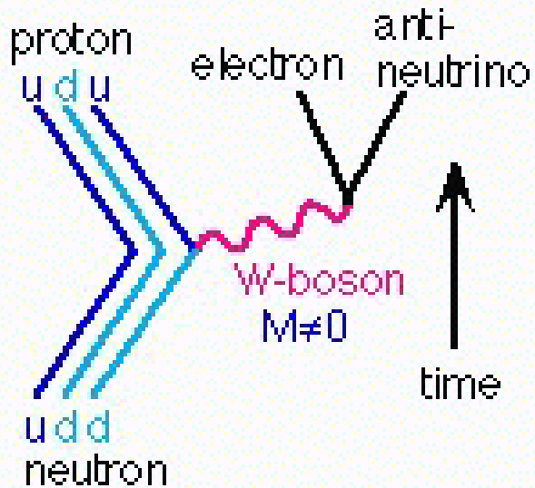
Decay of a neutron into a proton by the Weak force
