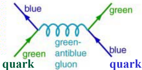
Strong Force
